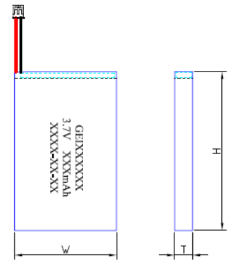
Dimension(without PCM and wire) T: 5.8mm W: 34mm H: 50mm (Note:Drawings just for reference)
