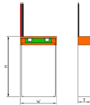
Dimension(without PCM and wire) T: 5.2mm W: 34mm H: 50mm (Note: Drawings just for reference)
