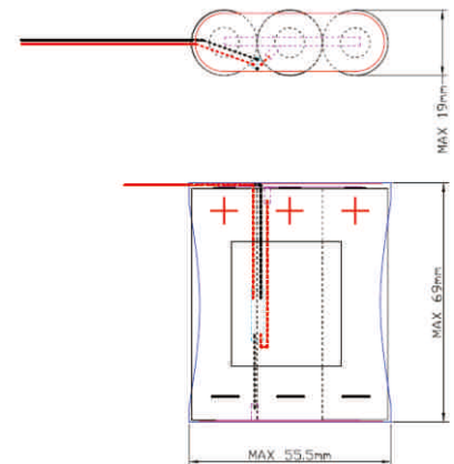
Thickness: 19mm Width: 55.5mm Height: 69mm
